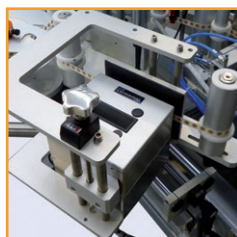
Thermal transfer coding unit
